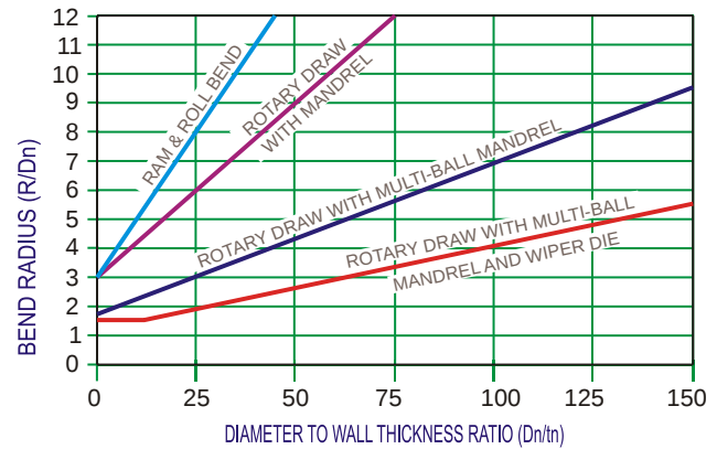
FIGURE 6.8.1 COLD BENDING RANGE
