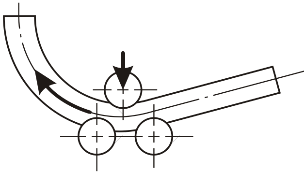
FIGURE 3.5.3 ROLL BENDING
