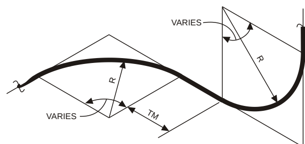
FIGURE 7.5.4 TANGENT LENGTHS
