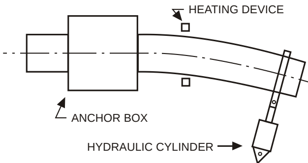
FIGURE 3.4.2 INCREMENTAL BENDING
