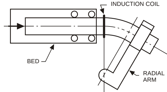
FIGURE 3.4.3 INDUCTION BENDING
