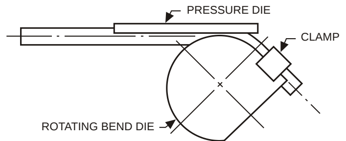
FIGURE 3.5.1 ROTARY DRAW BENDING
